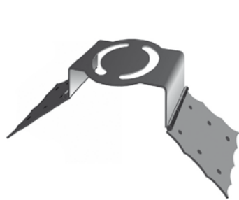
Fixierplatte schwarz 55.13.0402
