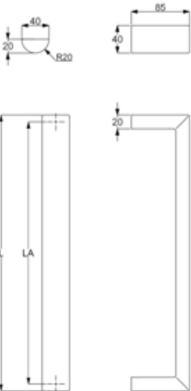
Push handle without mounting hardware and mounting accessories, support straight
