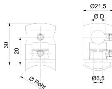
Stainless steel grain 240 matt, 2-part (flexible)
