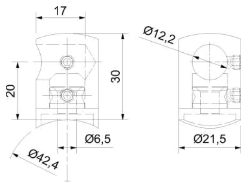
Stainless steel grain 240 matt, with blind hole 12,2 mm, 2-part (flexible), with attachment for pipe Ø 42,4 mm
